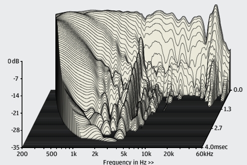
ABOVE: Cabinet resonances are quickly suppressed. The main 'feature' is associated with the 3.9kHz notch
